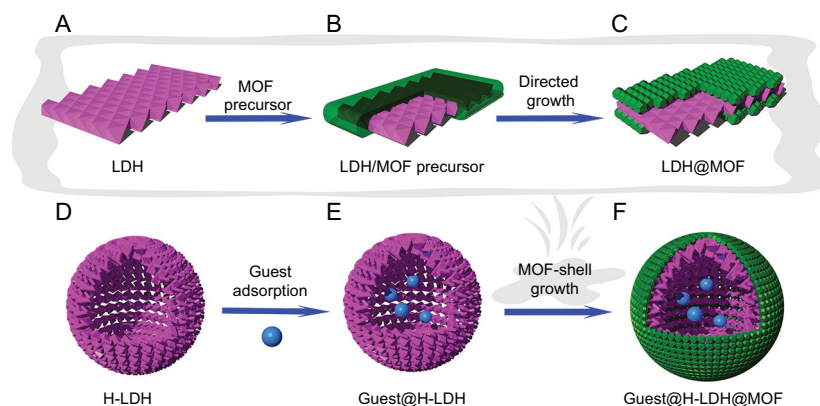
Figure 1. Schematic for the fabrication of the yolk-shell MOF capsule. (A–C) The template-assisted strategy to create LDH@MOF and (D–F) encasing guest molecules (blue sphere) into H-LDH by creating a yolk-shell MOF capsule. Redrawn from Fig. 2 of [4].
