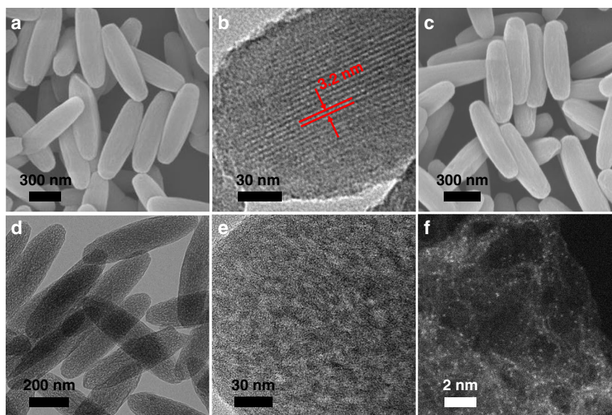
Fig. 2 Microscopic characterizations. a Scanning electron microscopy (SEM) and b transmission electron microscopy (TEM) images of PCN-222(Fe). c SEM and d TEM images of \text{Fe}_{\text{SA}}\text{-N-C} . e Enlarged TEM image showing the mesoporous structure of \text{Fe}_{\text{SA}}\text{-N-C} . f Aberration-corrected HAADF-STEM image of \text{Fe}_{\text{SA}}\text{-N-C} .
