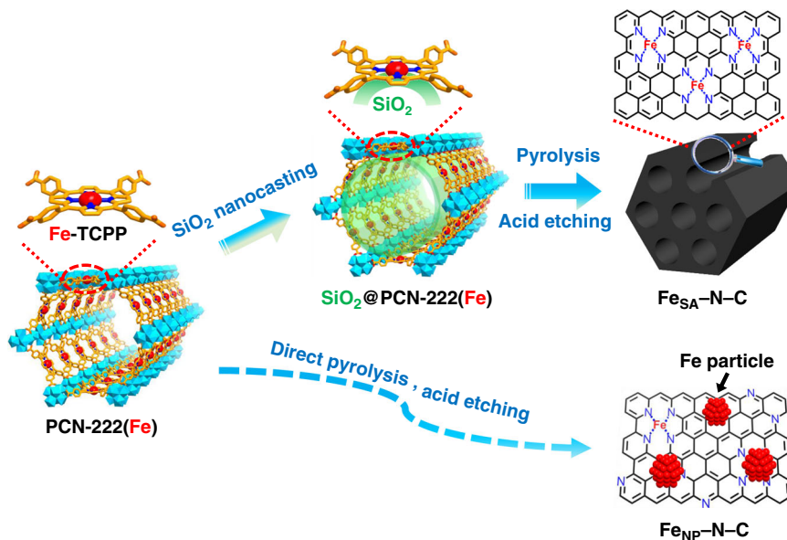
Fig. 1 Schematic illustration. Illustration showing the nanocasting-assisted fabrication of \text{Fe}_{\text{SA}}\text{-N-C} from PCN-222(Fe).
